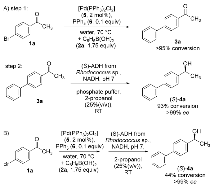
Scheme 2. Synthesis in two separate steps (A) versus one-pot two-step synthesis (B).
