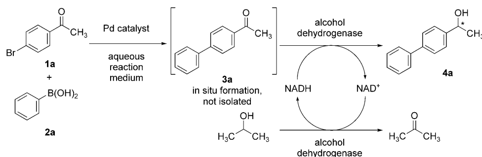
Scheme 1. Concept of the chemoenzymatic one-pot synthesis. NAD + = nicotinamide adenine dinucleotide; NADH is the reduced form of NAD + .
