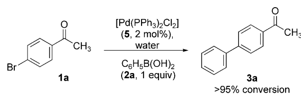
Scheme 3. Optimized Suzuki cross-coupling in water.
