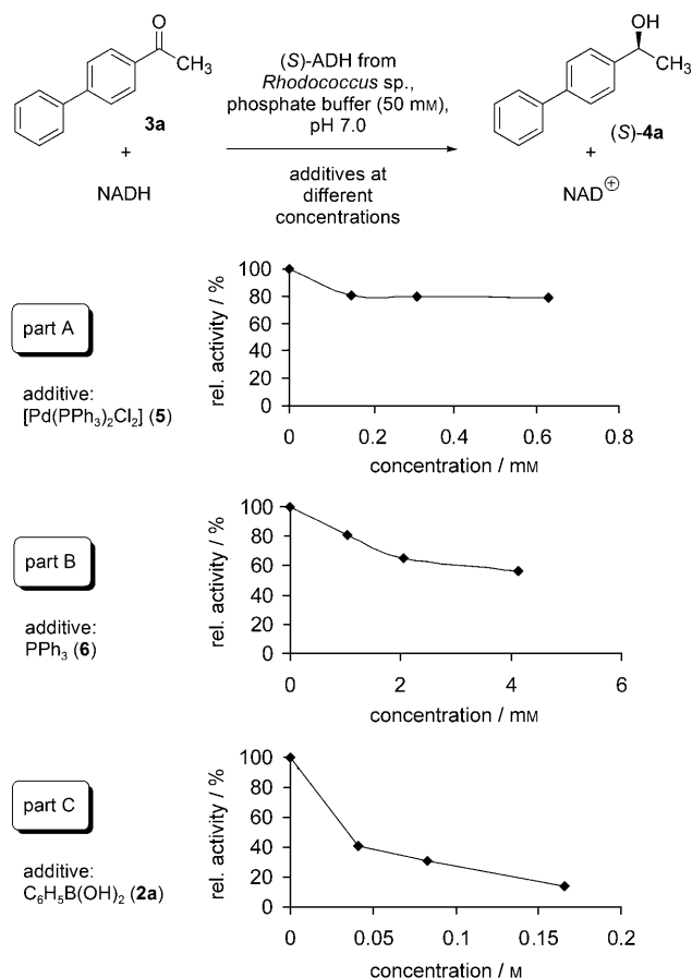
Figure 1. Influence of the components of the Suzuki cross-coupling on enzyme activity.
