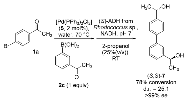
Scheme 4. Synthesis of the enantiomerically pure diol (S,S)- 7 .
